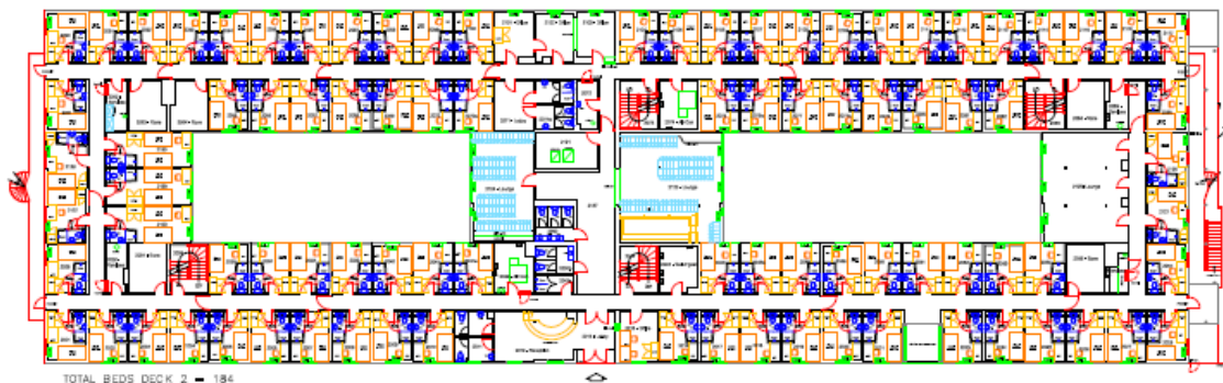
PLAN VIEW ON DECK 2 SCALE 1:150
