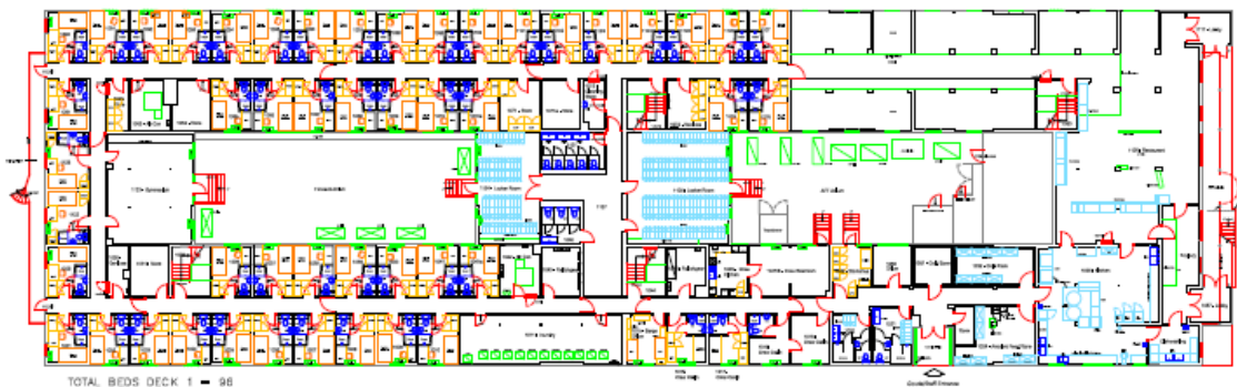
PLAN VIEW ON DECK 1 SCALE 1:150
